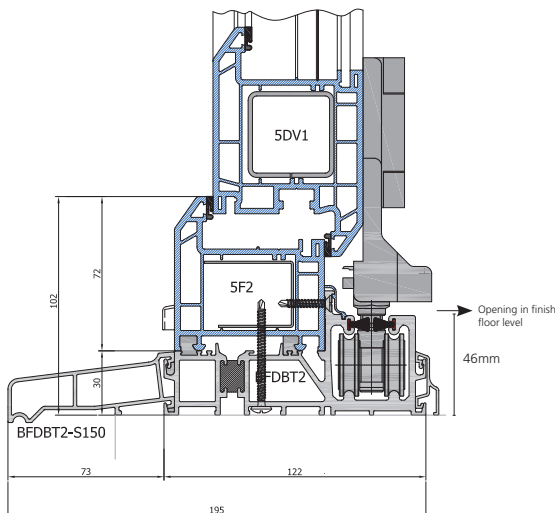
DOOR OPENS IN 150mm Sill Nose
