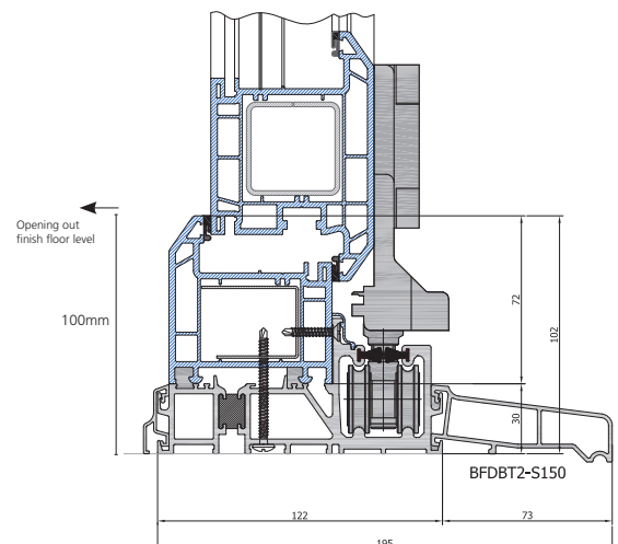
DOOR OPENS OUT 150mm Sill Nose
